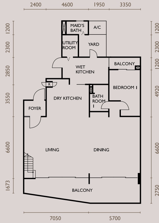
TYPE D4 - LOWER
